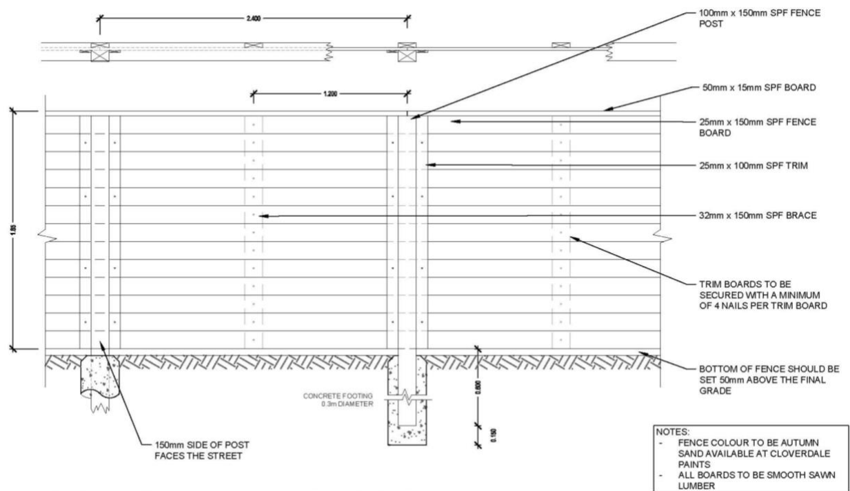
HORIZONTAL SLAT WOOD SCREEN FENCE DETAIL
