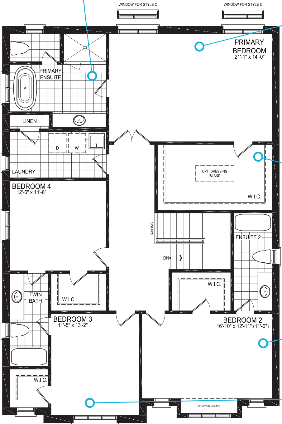
SECOND FLOOR STYLE B
